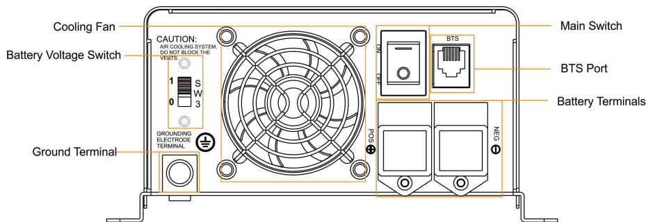
Figure 1 Front Panel
