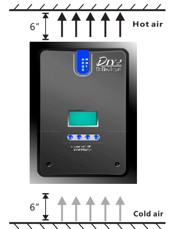
Fig. 2.1 Installation and heat dissipation
