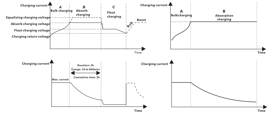
Fig. 1-5 SLD Battery charging stages diagram
