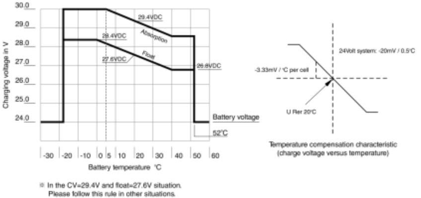
Figure 11. CX24xx model Temperature Compensation
