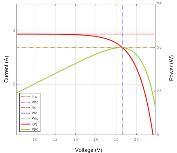
RNG-50D-SS Characteristics Versus Voltage
