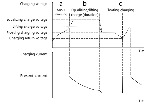
Charging Curve of Lead-Acid Battery
