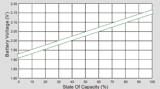
Relationship of OCV And State of Charge(20°C)
